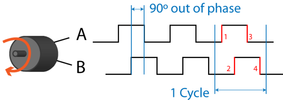
Signal A and B in Quadrature
