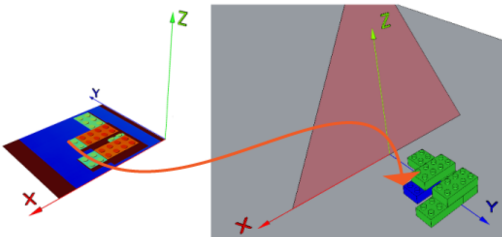
Transformation from Image 3D to Sensor 3D Space
